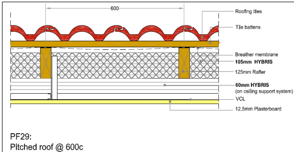
Figure 3: Typical HYBRIS Installation with Two Layers
